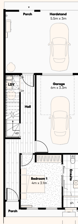
Ground floor
