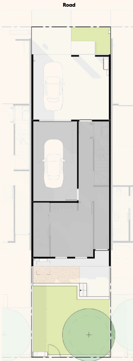
Site plan
