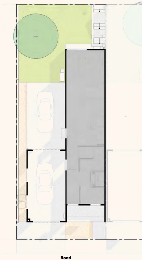
Site plan
