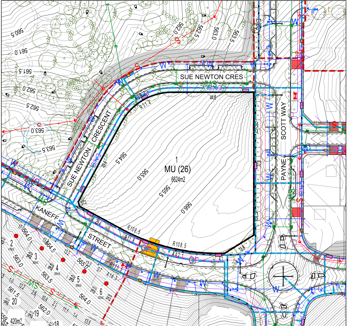
BLOCK LAYOUT - SCALE 1:1000
