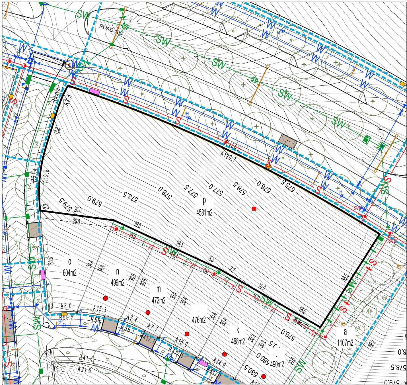
BLOCK LAYOUT - SCALE 1: 750
