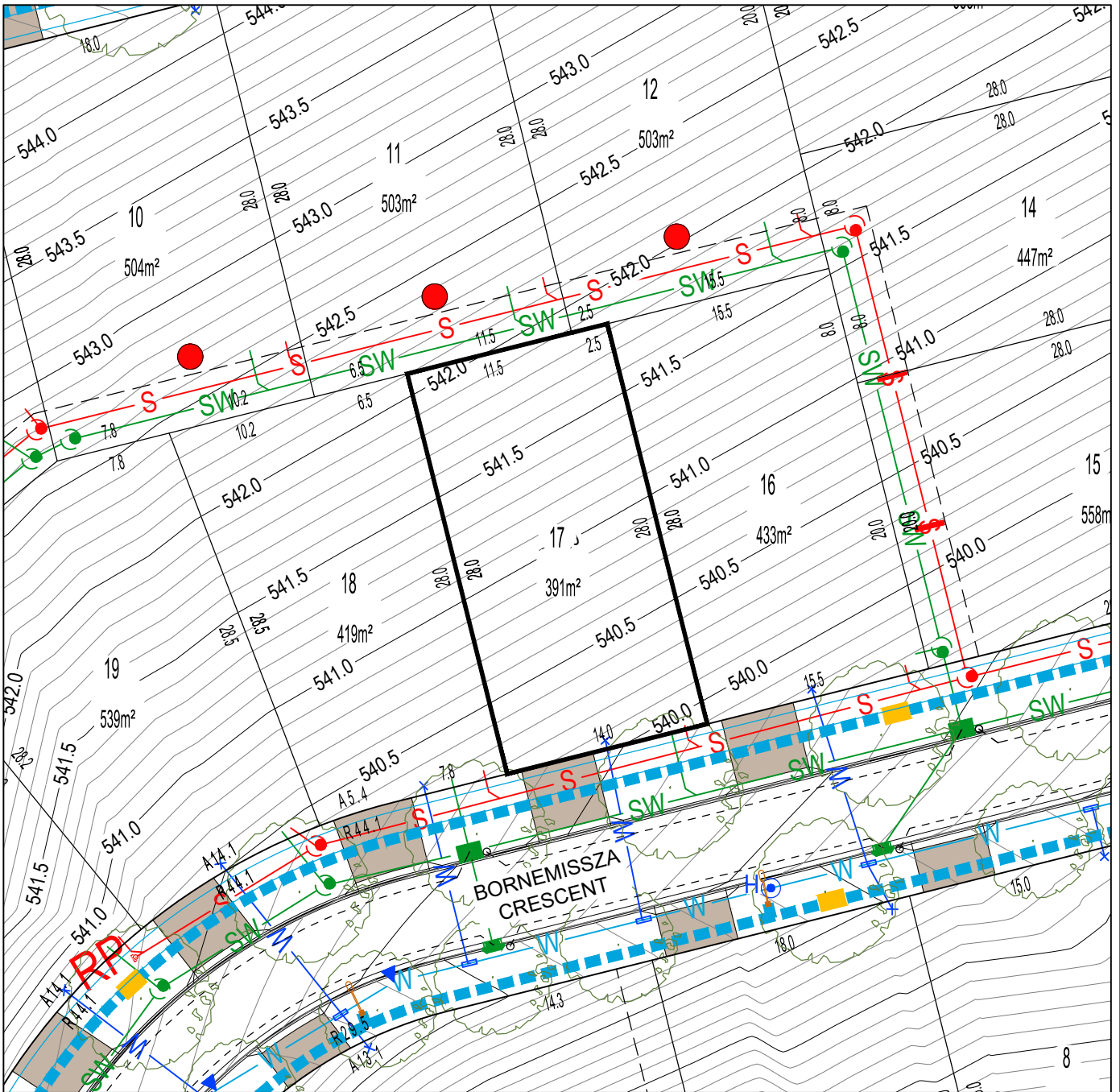
BLOCK LAYOUT - SCALE 1:400
