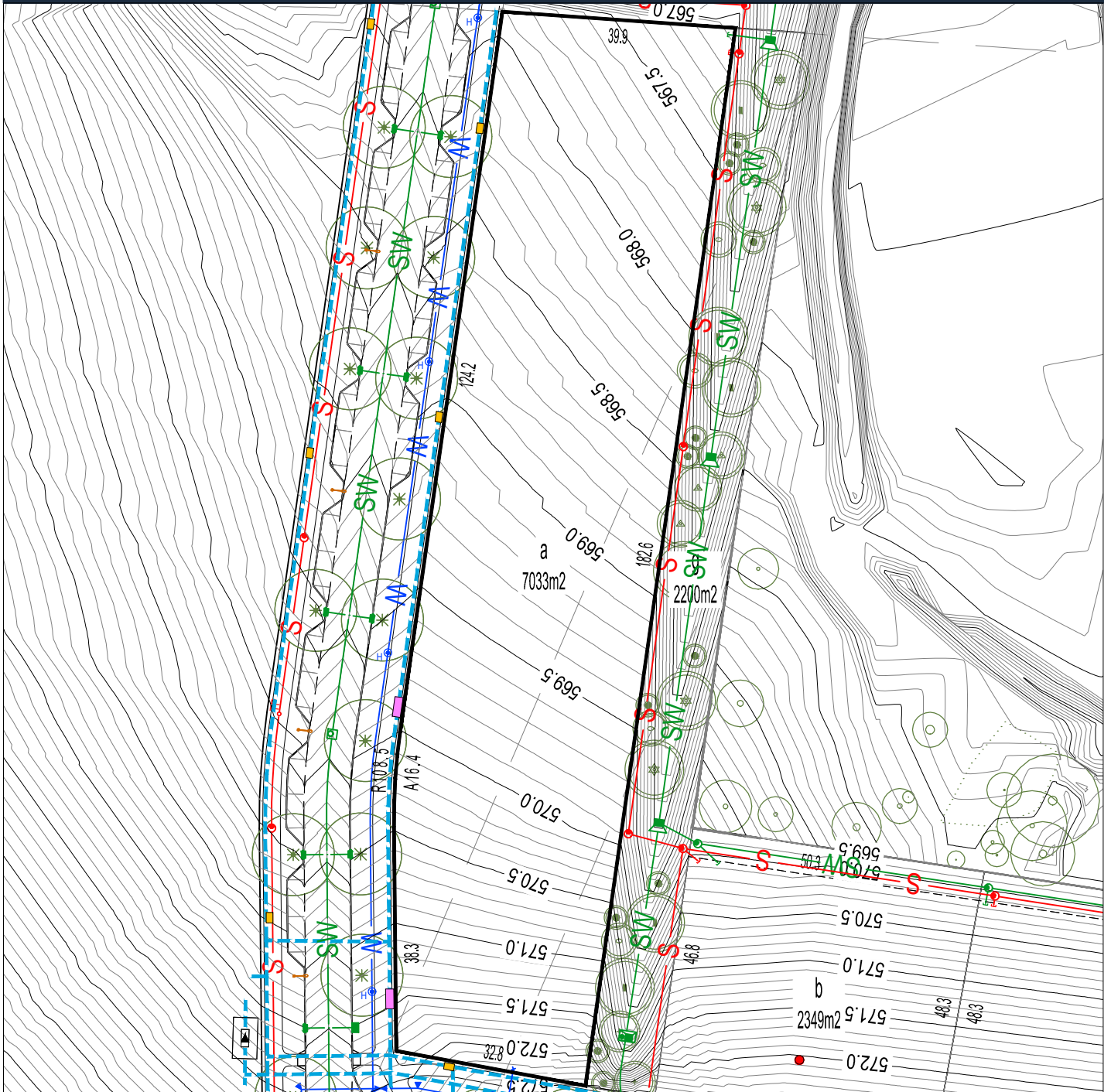
BLOCK LAYOUT - SCALE 1:1000
